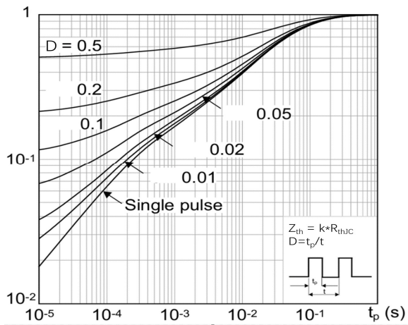
Fig.11 Max transient thermal impedance for Diode
