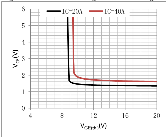
Fig.7 Collector-Emitter VS gate source voltage
