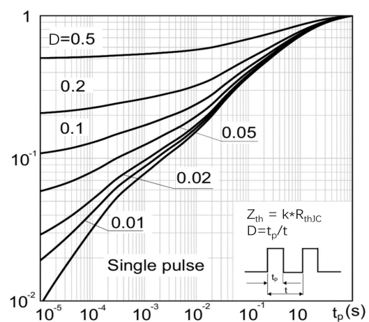
Fig.10 Max transient thermal impedance for IGBT
